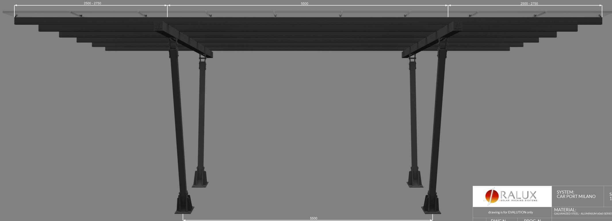
FRONT VIEW
