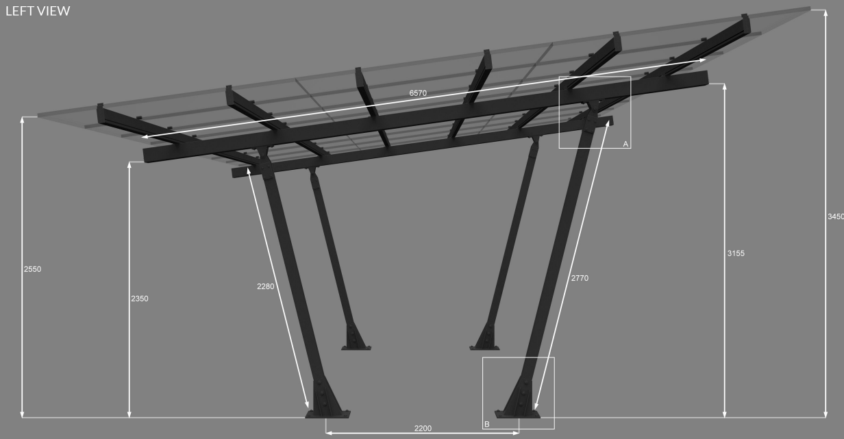
LEFT VIEW
